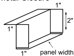
Metal Closure
