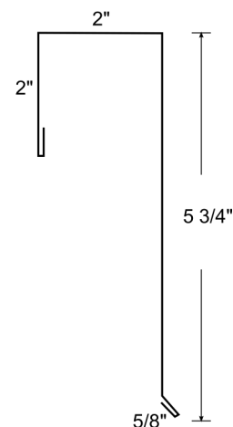
Gable Trim
