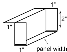
Metal Closure
