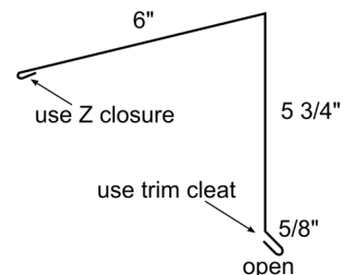
Top Shed
