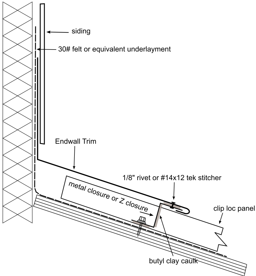
Z Closure
